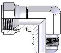
Tournant JIC x Male JIC 90° 90° JIC Swivel x JIC Male
